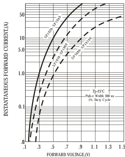
FIG.2-TYPICAL FORWARD CHARACTERISTICS
